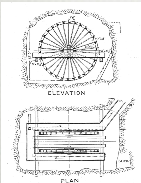
DRAINAGE WHEEL FROM RIO TINTO MINES
