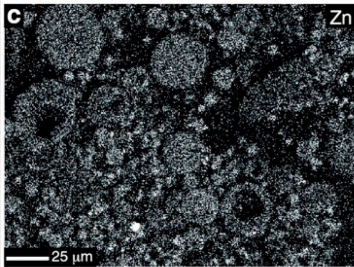
Backscattered electron image and element distribution maps for an area studied in detail by EPMA. (a) BSE image; (b), (c), and (d) are X-ray maps that show the distributions Cu, Zn, and U, respectively. Bright particles in the BSE image are Fe-rich spheres. Particles with numbers to their immediate left are discussed in the text.
