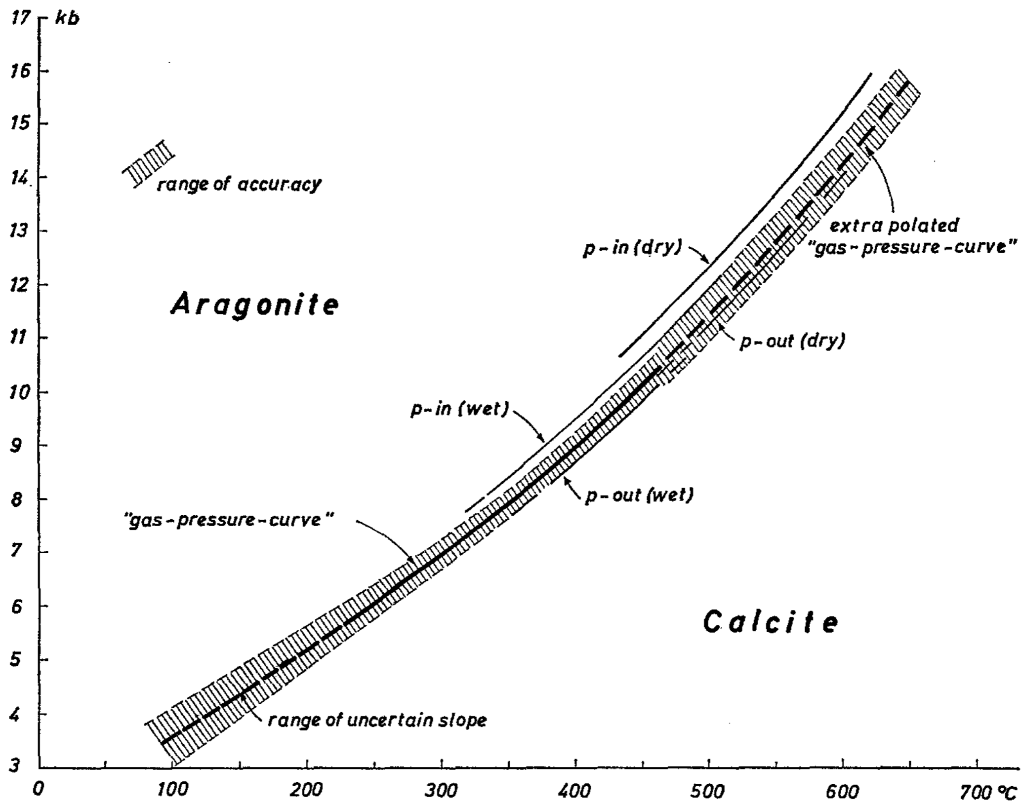
Fig. 4. Composition of piston-cylinder and gas-pressure runs
