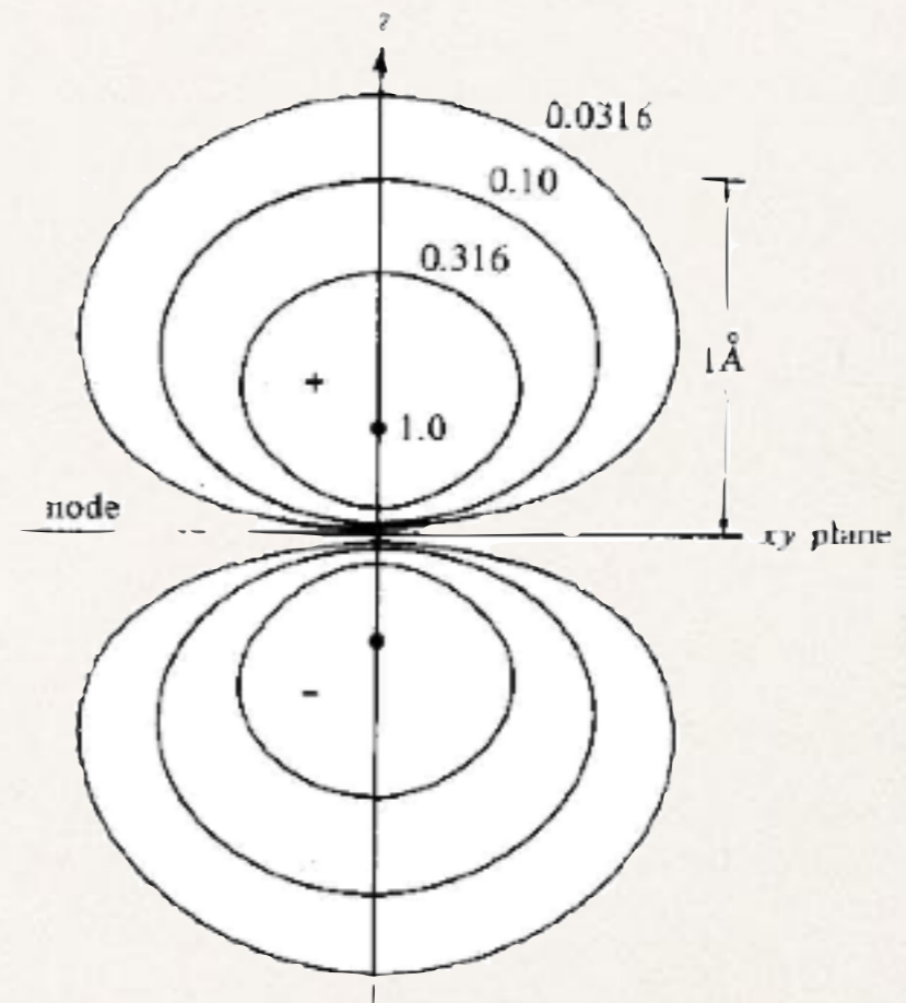
Electron density contours for hydrogen-like 2p_z orbital of carbon. Contour values are relative to the electron density maximum. The x-y plane is a nodal surface. The signs (+ and -) refer to the original wave function, \Psi .
