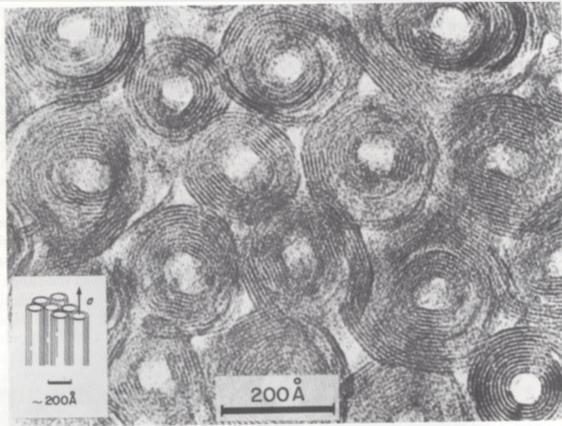
Figure 6. Transmission electron micrograph of the cross-sections (perpendicular to the fiber axis) of chrysotile fibers. Specimen from the Transvaal Province, South Africa (photograph reproduced with permission from Plate 46 in Sudo et al., 1981, Electron Micrographs of Clay Minerals , Elsevier, Amsterdam). Insert is a sketch of the packing of chrysotile fibrils parallel to the a crystallographic axis. Compare with Figures 8, 9, 12, and 13 in the chapter by Veblin and Wylie, this volume.
