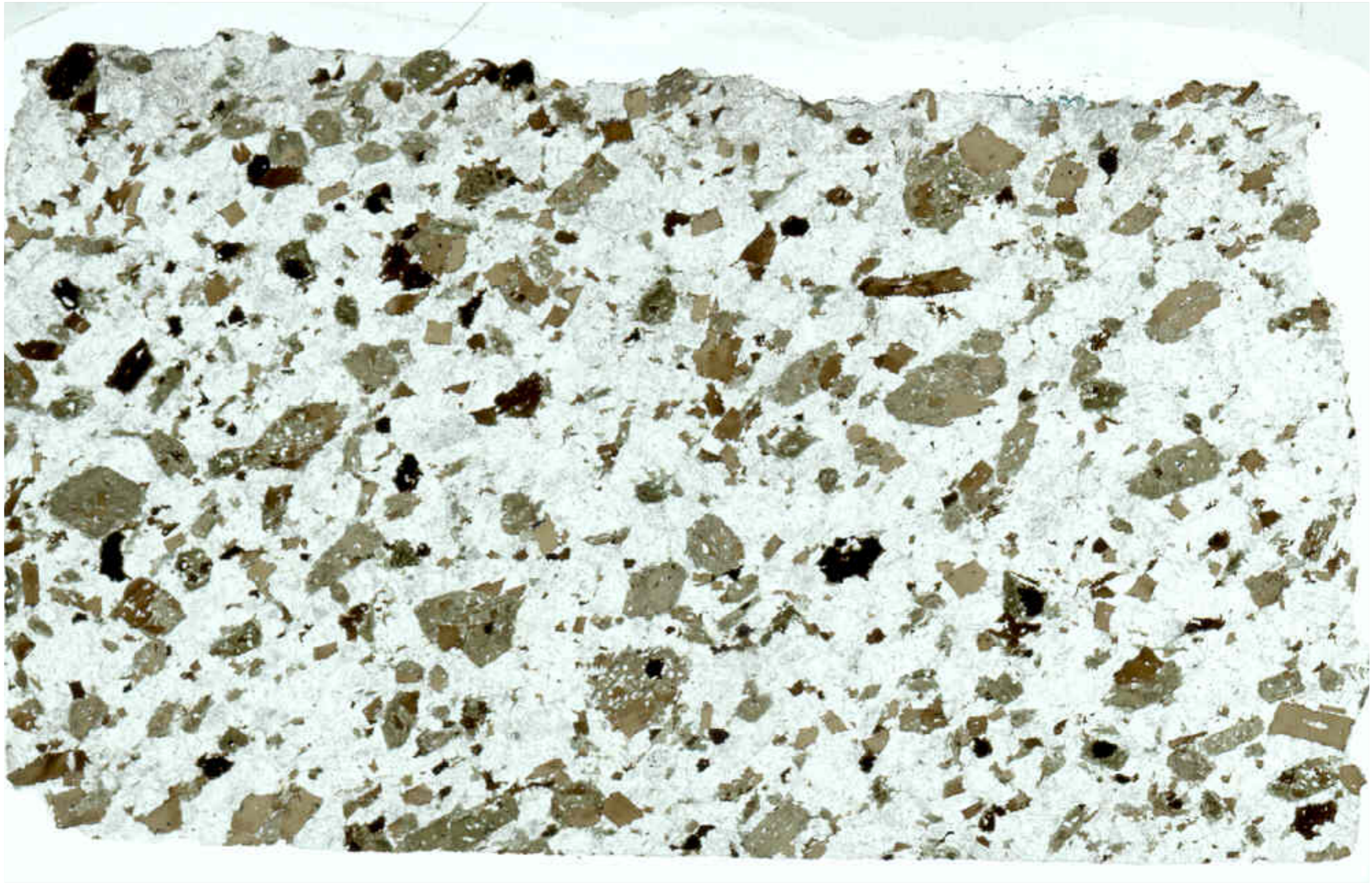
Hornblende diorite, Malaysia
