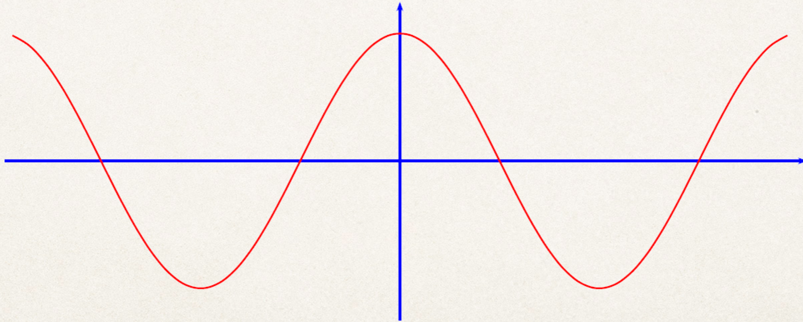
Figure 5: Cosine function.
