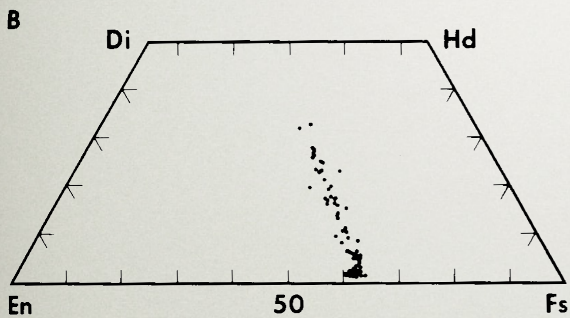
1.2.8.4 Pyroxene compositions in basaltic meteorites. a. Pasamonte, an unequilibrated eucrite. b. Stannern, an equilibrated eucrite. c. Three cumulate eucrites (BD-Binda, MA-Moama, MC-Moore County) plus one main group eucrite (JV-Juvinas). Open circles represent bulk compositions of pyroxenes; filled circles represent exsolution lamellae. d. Shergotty.
