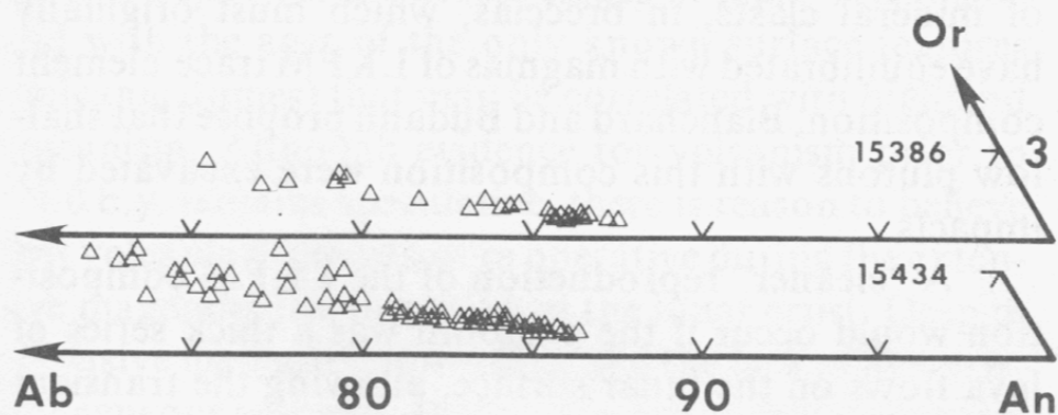
1.2.10.5 Ab-An-Or composition of feldspars in LKFM and IKFM samples. Data from this study, and from the sources cited for Fig. 1.2.10.4. Note that the use of various symbols denotes textural differences within poikilitic samples.
