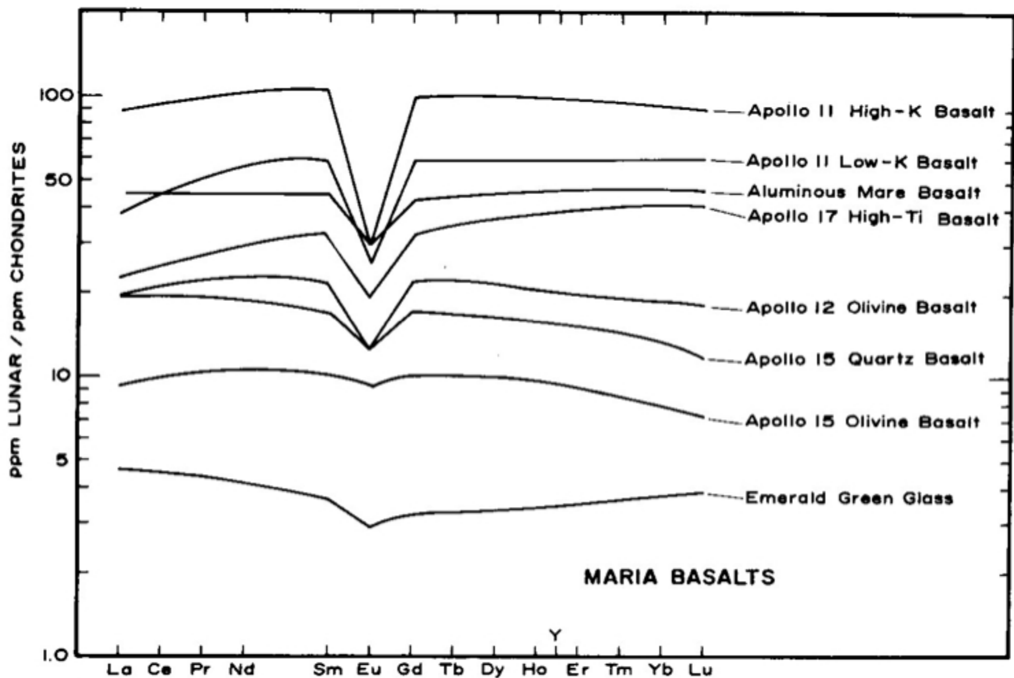
Fig. 4.22 Rare earth patterns for maria basalts, plotted relative to chondritic abundances [60]. Note the variable degree of europium depletion and the tendency for the light rare earths (La-Sm) to decrease relative to the chondritic abundances.
