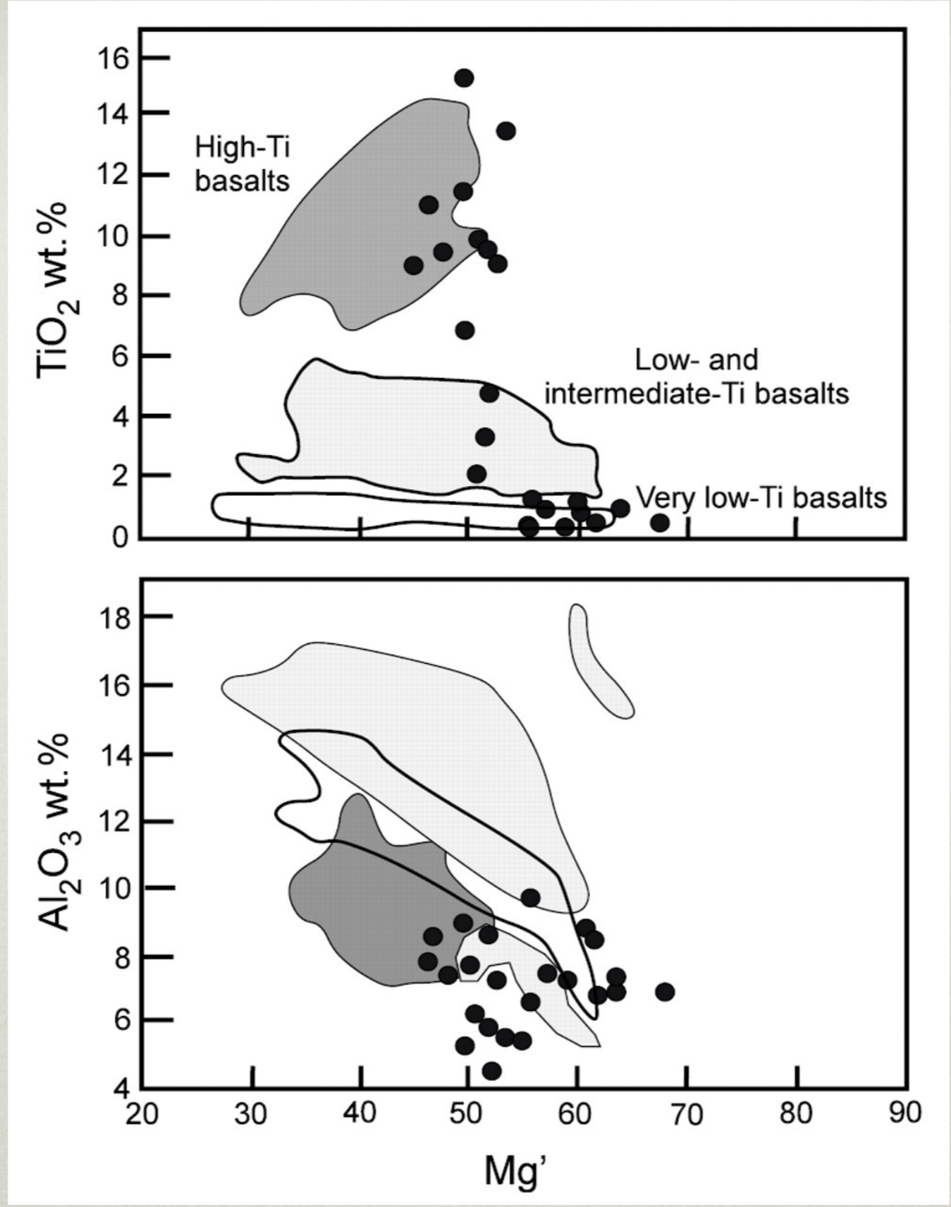
Mg' values vs. TiO 2 and Al 2 O 3 for mare basalts (enclosed fields) and picrite glasses filled circles (modified after Shearer and Papike 1993).
