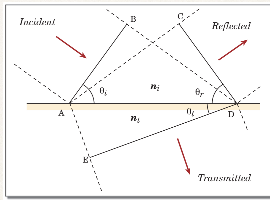
Law of refraction
